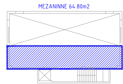
mezzanine esc :1:75
